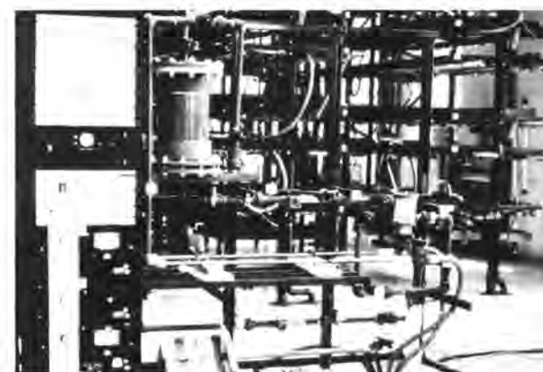
Equipment racks for biofouling and corrosion experiments.
