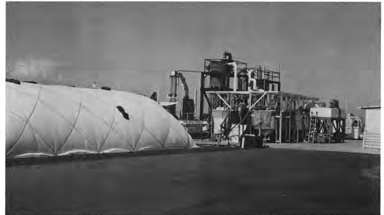
The Test Pad Area - Left to Right: Lobster aquaculture inflatable building, Mist-lift experimental apparatus, header tanks (behind), fish tanks (in front).
