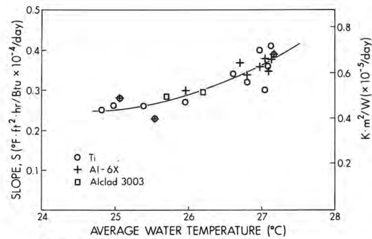
Figure 2. Fouling rate (s) as a function of average water temperature. Units for s are (^\circ\text{F}\cdot\text{ft}^2\cdot\text{hr}/\text{BTU})\times 10^{-4}/\text{day} (left hand scale) or (^\circ\text{C}\cdot\text{m}^2/\text{watt})\times 10^{-5}/\text{day} (right hand scale).
