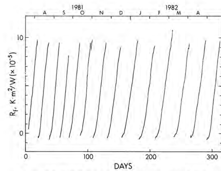
Figure 1. R_f vs time curves for free fouling titanium. R_f units are 10^{-5} \times ^\circ\text{C}\cdot\text{m}^2/\text{watt} .
