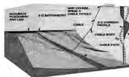
BELOW: Makai Ocean Engineering-- Cable Lay Software
